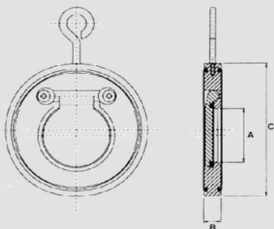
DIMENSIONS IN (MM) SERIES - 40 (SIZE 2" - 6")
